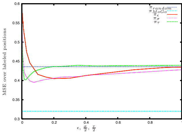
Figure 3. The MSE of each policy \pi when Monte Carlo simulation is used to evaluate a test suite of 200 hand-labelled positions. The x axis indicates the degree of randomness in the policy.
