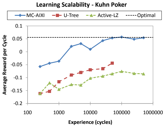
Figure 7: Average Reward per Cycle vs Experience
