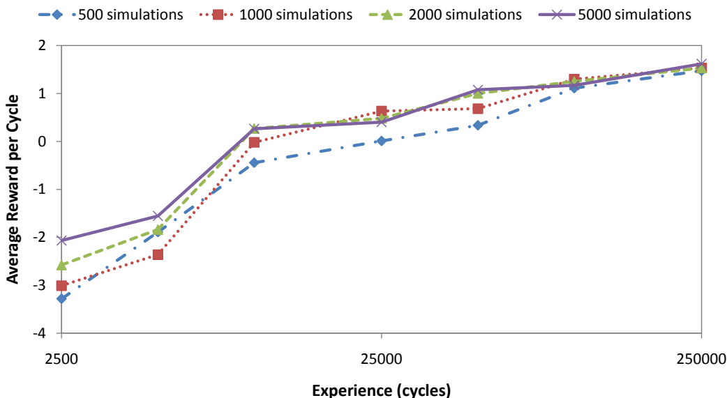
Figure 9: Scaling properties on a challenging domain
