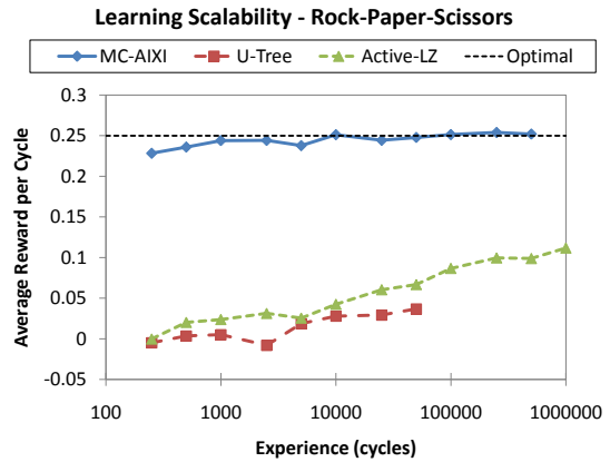
Figure 7: Average Reward per Cycle vs Experience
