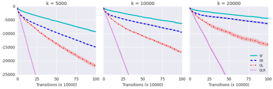
Figure 1: Cumulative return on the moving-puddles task. The parameter k above each plot indicates how often the reward function changes. Shaded regions represent one standard error over 30 runs.
