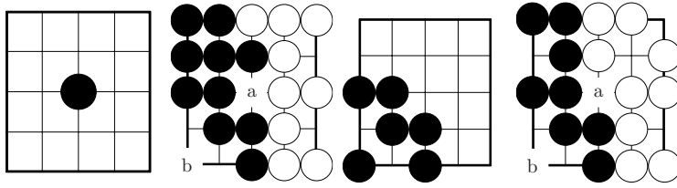
Fig. 12 a) A 1 \times 1 local shape feature with a central black stone. This feature acquires a strong positive value in the long-term memory. b) In this position, move b is the winning move. Using only 1 \times 1 local shape features, the long-term memory suggests that move a should be played. The short-term memory will quickly learn to correct this miscalculation, reducing the value of a and increasing the value of b . c) A 3 \times 3 local shape feature making two eyes in the corner. This feature acquires a positive value in the long-term memory. d) Black to play, using Chinese rules, move a is now the winning move. Using 3 \times 3 features, the long-term memory suggests move b , believing this to be a good shape in general. However, the short-term memory quickly realises that move b is redundant in this context (black already has two eyes) and learns to play the winning move at a .
