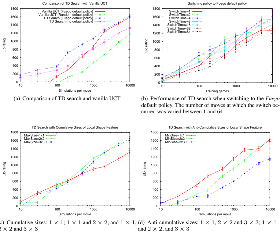
Fig. 7 TD search in 9 \times 9 Go.
