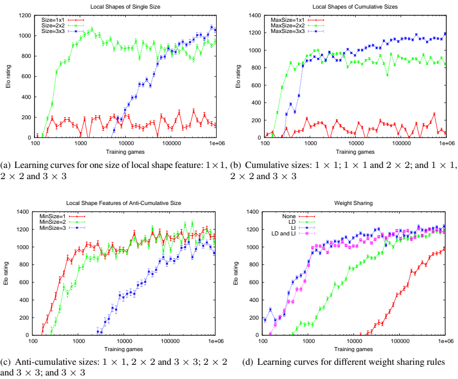
Fig. 5 TD learning in 9 \times 9 Go with different sets of local shape features.
